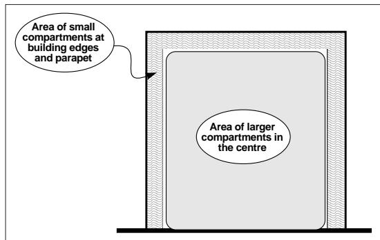
Figure 3. General pattern for façade compartmentation
